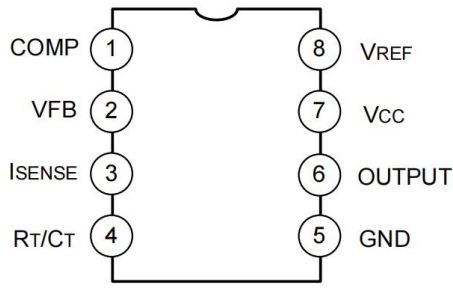
DIP-8/SOP-8
