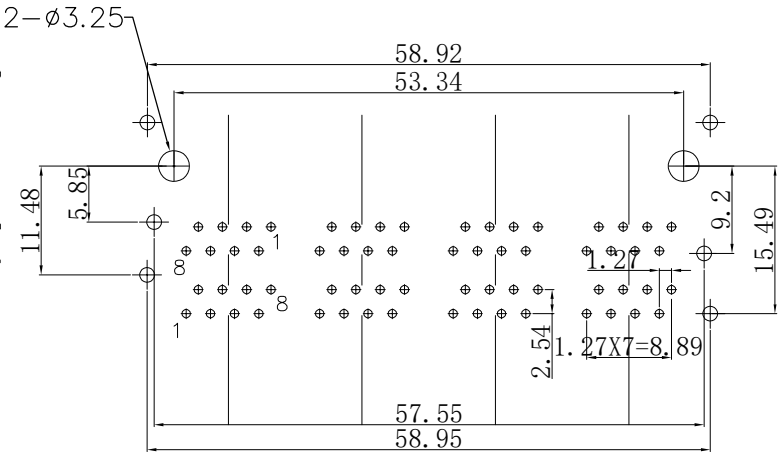
PC Board Layout Component Side Shown
