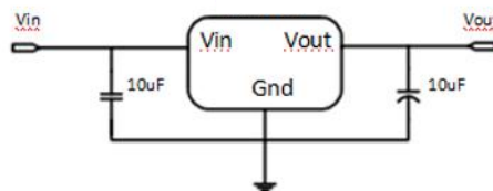
Application circuit of LD1117SxxTR fixed version
