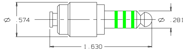
PLUG & SHIELD ASSEMBLY TP-108-6 (1 REQ'D)
