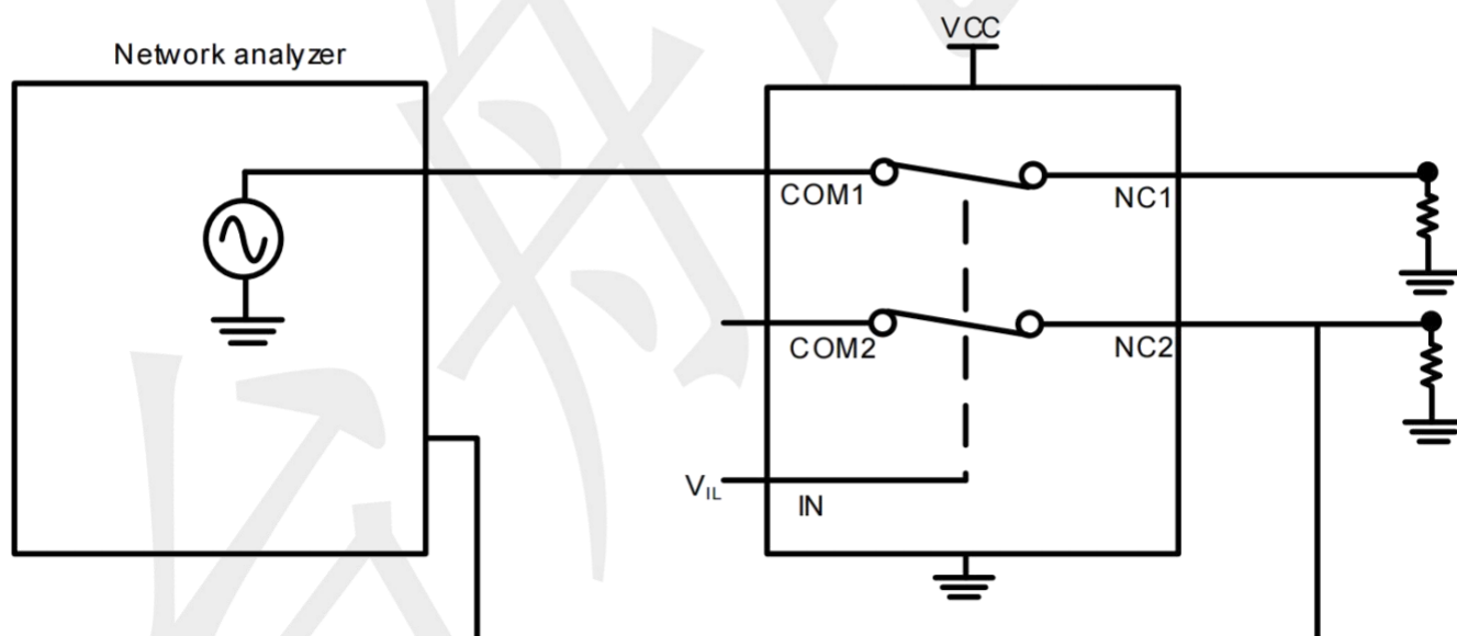
Crosstalk
