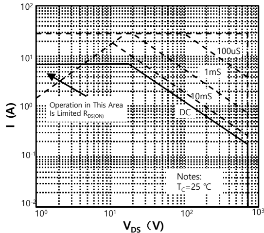
Figure 9-1. Maximum Safe Operating Area W TM08N65AD
