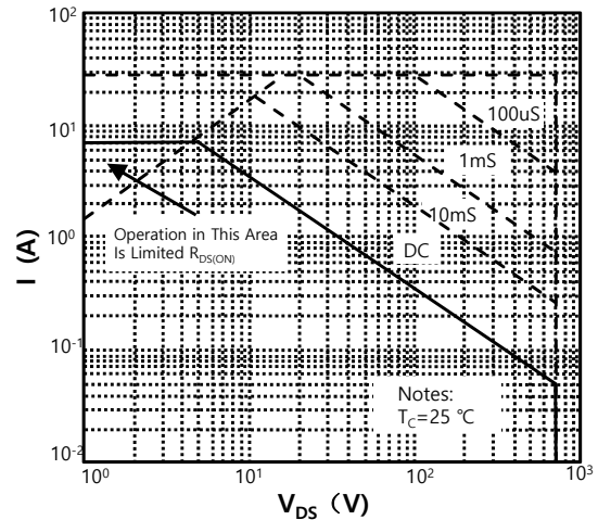
Figure 9-2. Maximum Safe Operating Area W TM08N65AF
