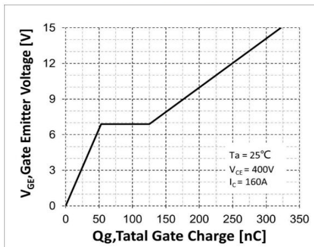
Fig.5 Gate charge
