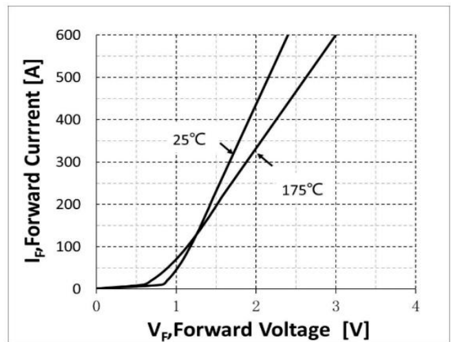
Fig.8 Typical diode VF vs. IF Characteristics
