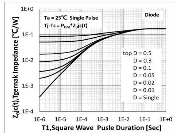
Fig.13 Transient Thermal Impedance Diode
