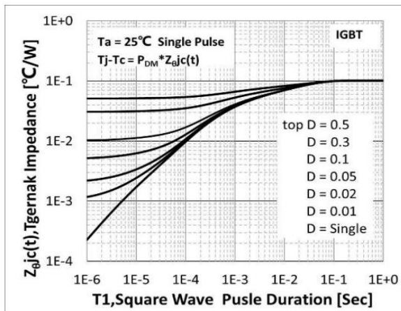
Fig.12 Transient Thermal Impedance IGBT
