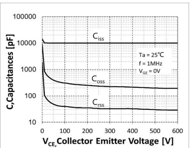
Fig.6 Typical capacitance
