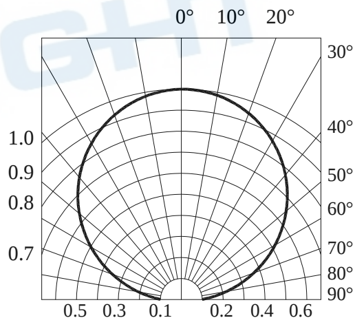
Fig.6 - Radiation Diagram
