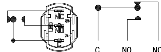
SCHEMATIC
