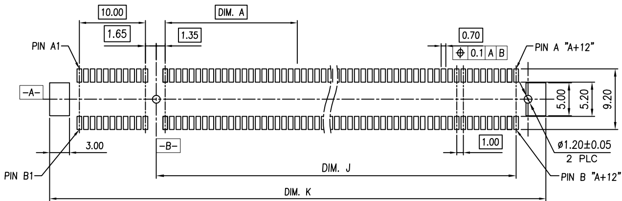
RECOMMENDED PCB LAYOUT (COMPONENT SIDE)
