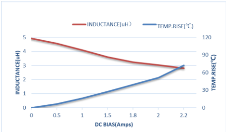
ZEMS201608-4R7M
