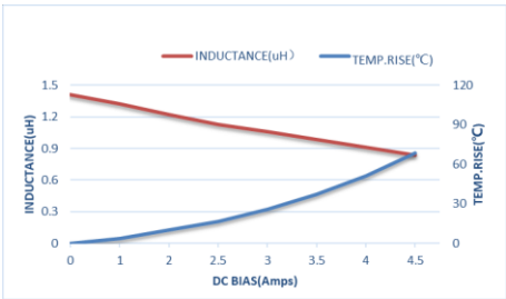
ZEMS201608-1R5M
