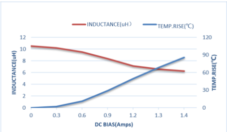
ZEMS201608-100M
