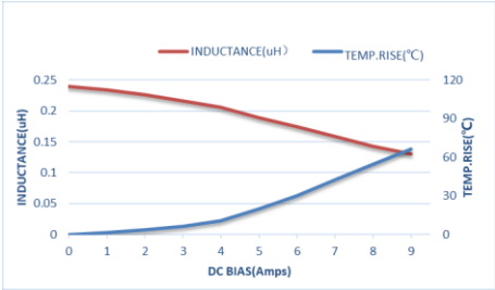
ZEMS201608-R24M
