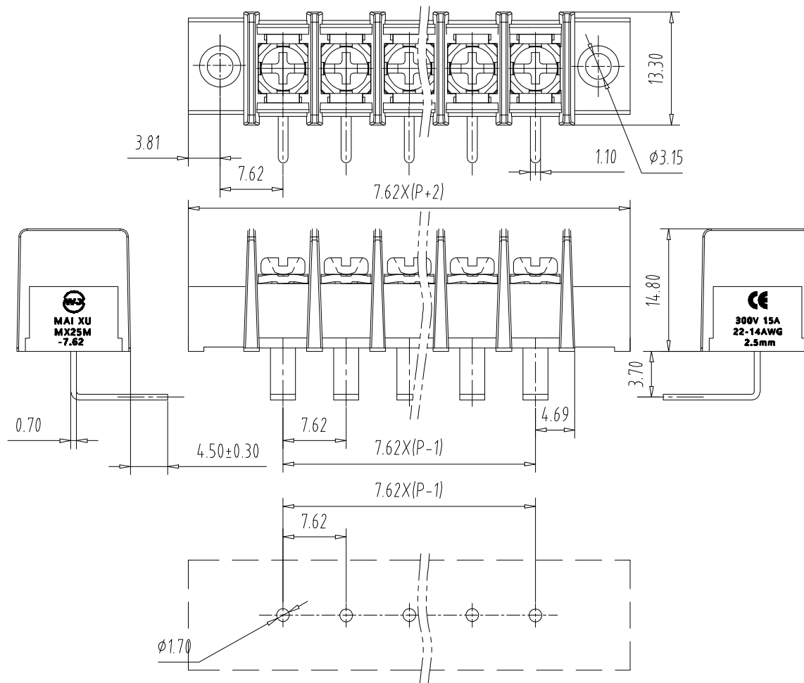
PCB Layout
