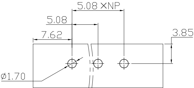
PCB LAYOUT
