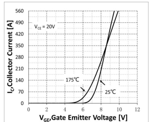
Fig.4 Transfer characteristics
