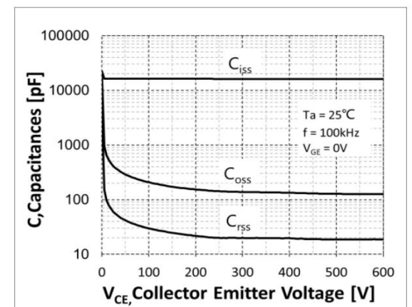
Fig.6 Typical capacitance
