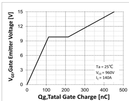
Fig.5 Gate charge
