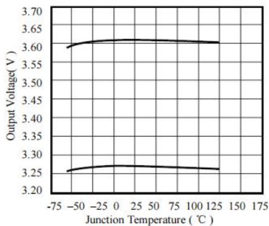
Figure 6. Output Voltage VS. Temperature
