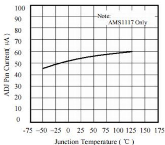
Figure 8. ADJ Pin Current VS. Temperature
