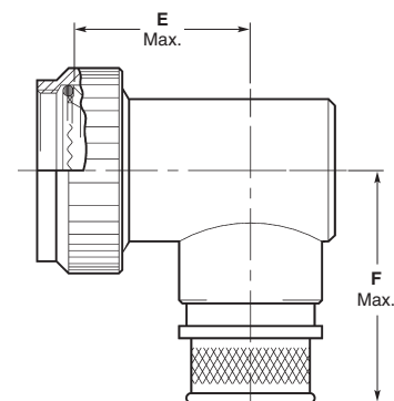
90° Adapter Code 90
