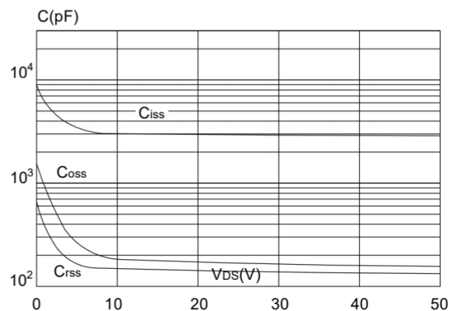
Figure 6: Capacitance Characteristics
