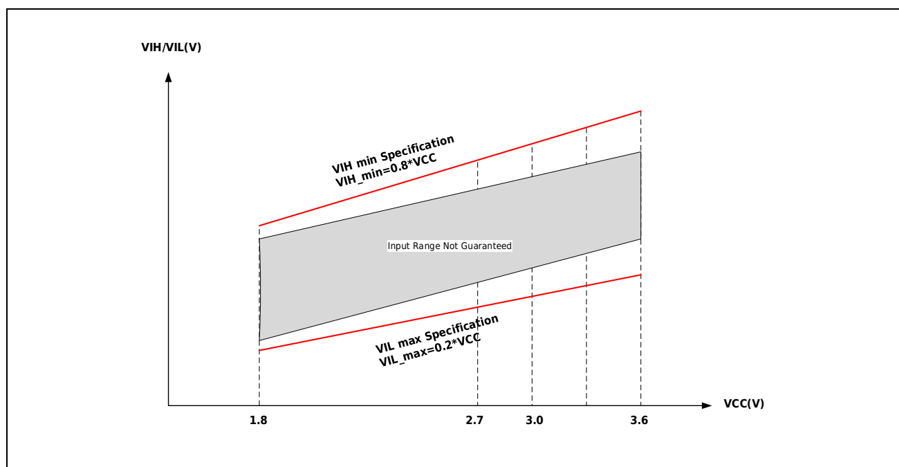
图 3-7 VIH/VIL versus VCC (Schmitt Input)
