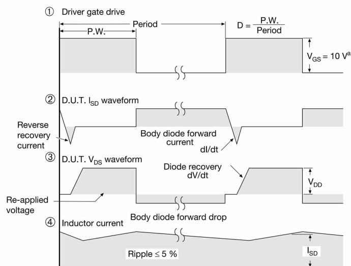
Fig. 14 - For N-Channel
