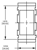
VMM MOUNTING PANEL MIDDLE
