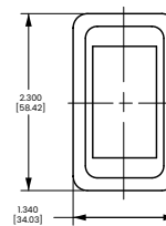
VMS MOUNTING PANEL
