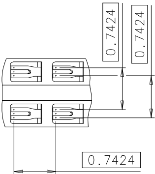
CONTACT DETAIL
