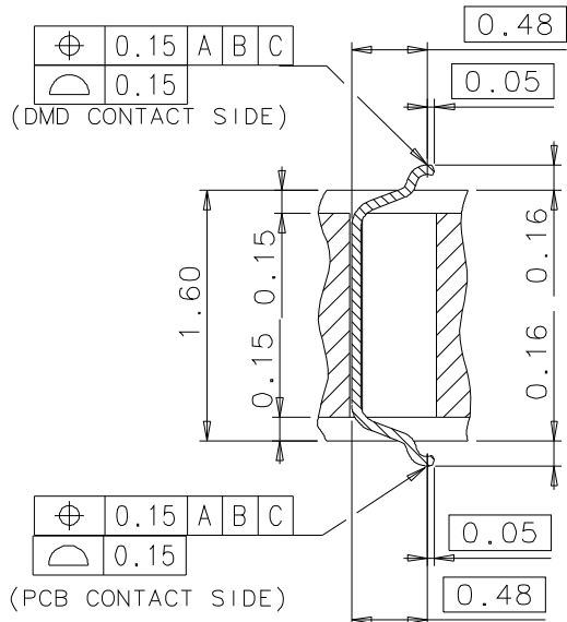
CONTACT CROSS SECTION DETAIL
