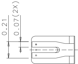
CONTACT DETAIL
