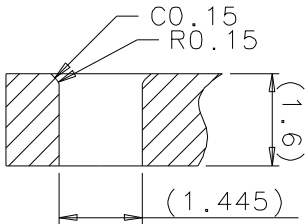
SECTION E-E
