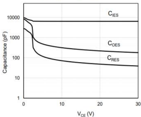
Fig.6 Typical capacitance
