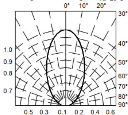
Fig.6-Radiation Diagram T_a=25^{\circ}\text{C}
