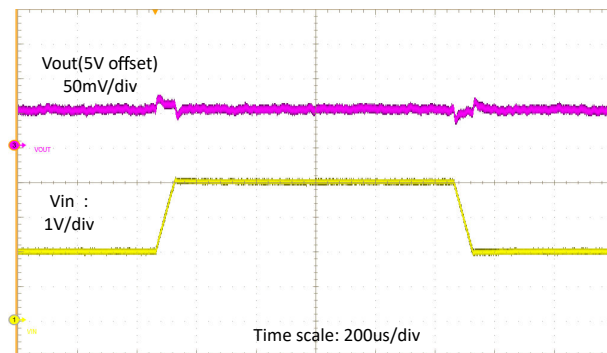
V_{IN} = 2V 至 4V , 20\mu s 转换率, V_{OUT} = 5V , R_{load} = 50\Omega
