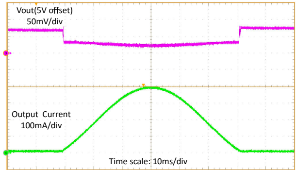
V_{IN} = 3.6V , V_{OUT} = 5V , I_{OUT} = 0mA 至 400mA 扫描
