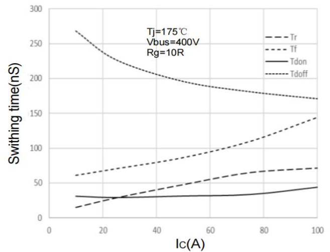
Figure 4:Switching time(nS)
