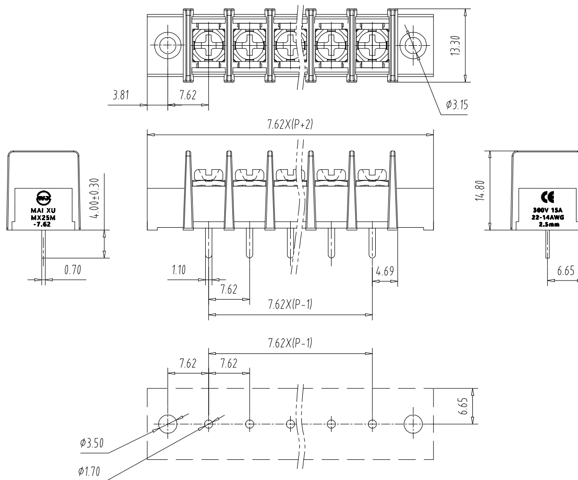
PCB Layout
