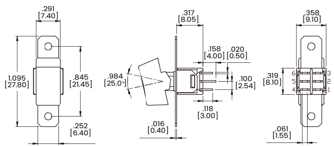
Double Pole
