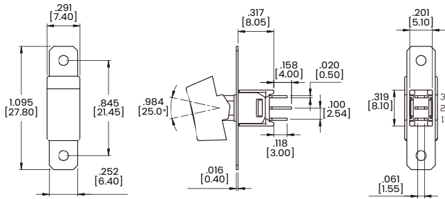
Single Pole
