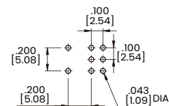
P.C.MOUNTING
