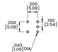
P.C.MOUNTING
