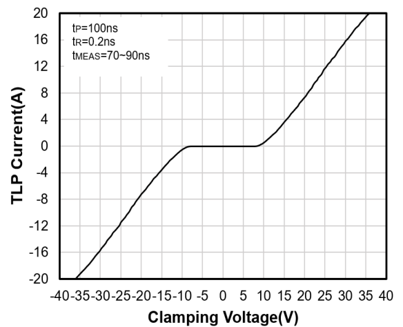
TLP Curve
