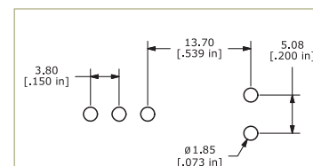
P.C. MOUNTING
