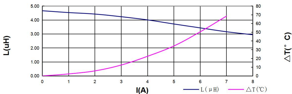
CURRENT CHARACTERISTIC
