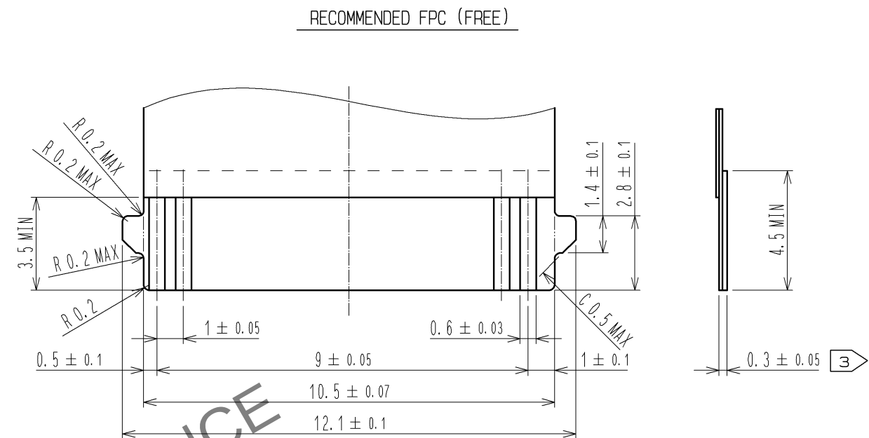
RECOMMENDED LAND PATTERN, METAL MASK(FREE)
