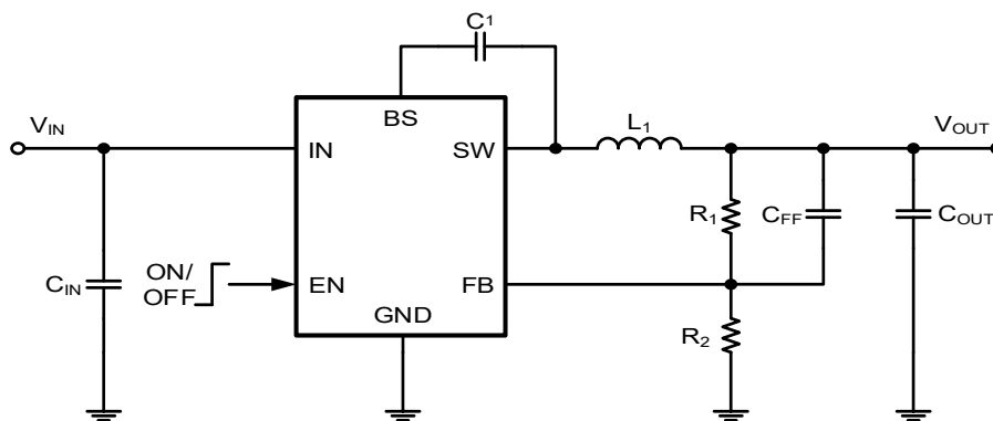
Basic Application Circuit
