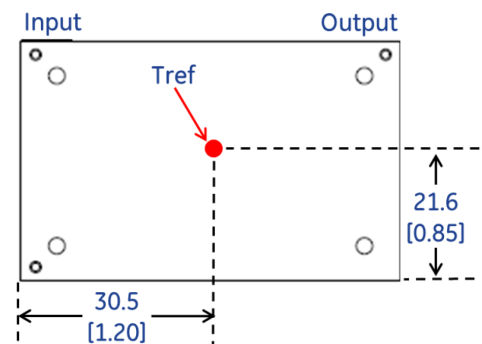
Figure 15. Location of the thermal reference temperature T_{ref} for base plate module.
