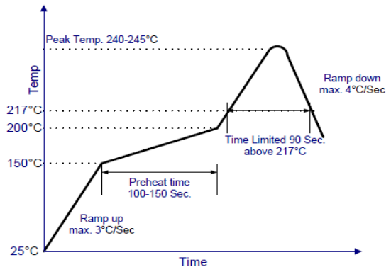
Figure 21. Recommended linear reflow profile using Sn/Ag/Cu solder
