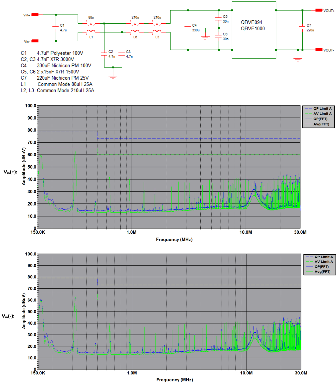
Figure 22. EMC Consideration
