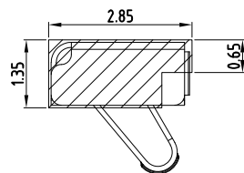
RECOMMENDED PCB LAYOUT TOLERANCE±0.05(焊盘推荐图)
