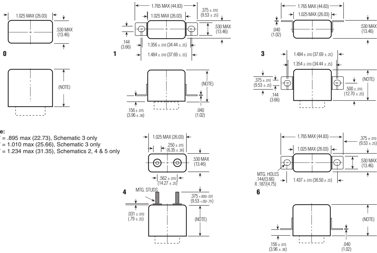
07 Mounting Styles
