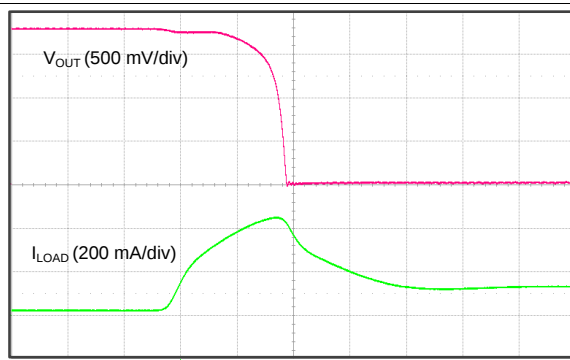
Time (100 \mu\text{s}/\text{div} ) TLV74318PDBV, 1\text{-}\mu\text{F} output capacitor
