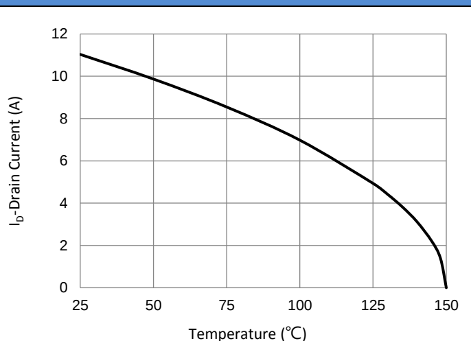
Fig.10 Drain Current vs. Case Temperature
