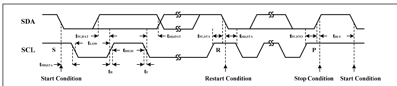
Figure 2 Interface Timing
