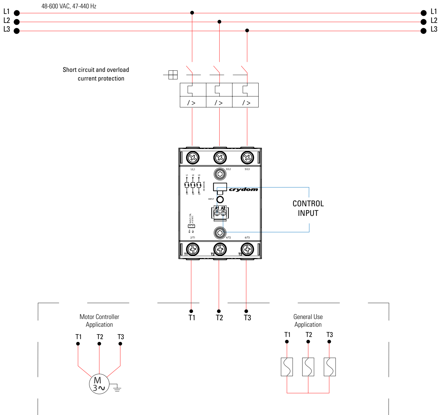
PM6760X(30,55,75) ( 2 CONTROLLED LEGS )
