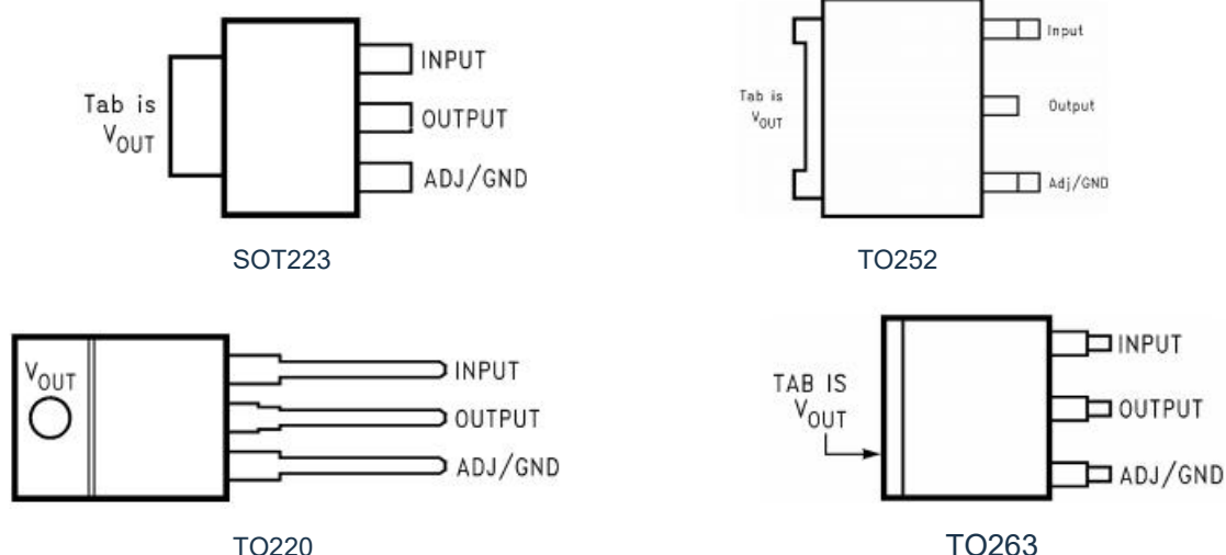
Figure 2.1: Top View
