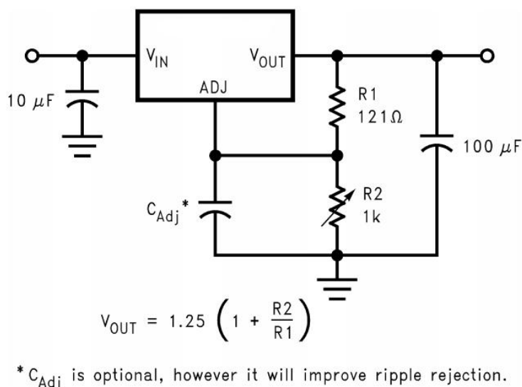
Figure 5.1. 1.25-V to 10-V Adjustable Regulator With Improved Ripple Rejection
