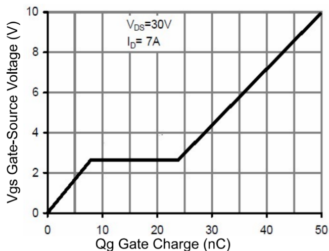
Figure 5 Gate Chare
