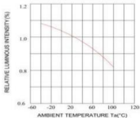
◆ 温度与亮度关系 (Temperature and brightness characteristic)
