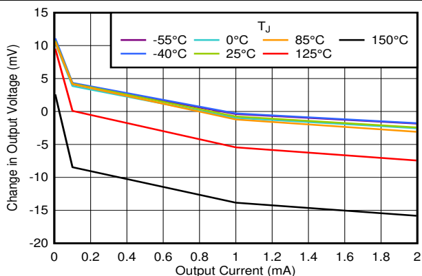
图 5-8. Load Regulation vs I_{OUT}
