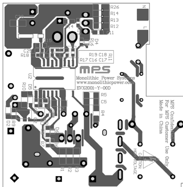
Figure 2: Bottom Layer – Main Power Board
