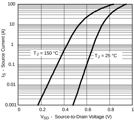
Forward Diode Voltage vs. Temperature
