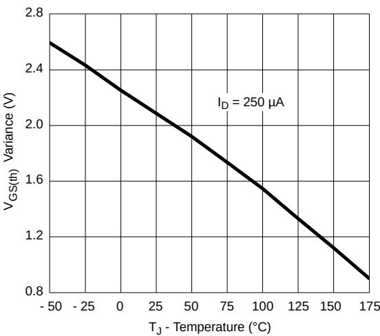
Threshold Voltage
