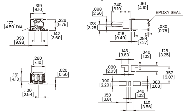
M6 Single Pole
