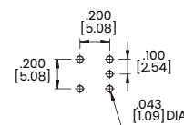
P.C. MOUNTING
