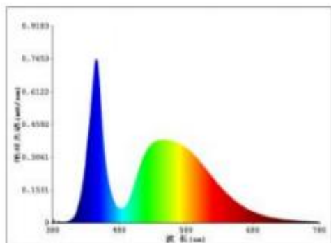
◆ 发射光谱 (Emission spectrum)
