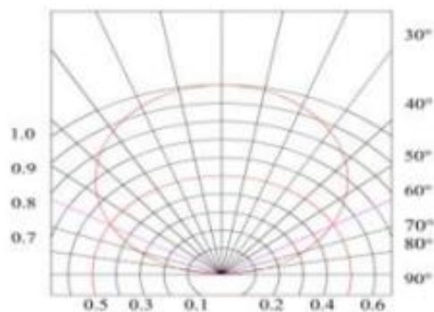
◆ 典型辐射分布图 (Typical radiation distribution map)
