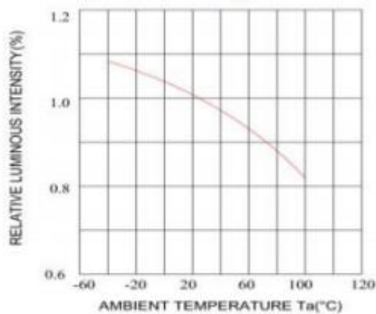
◆ 温度与亮度关系 (Temperature and brightness characteristic)
