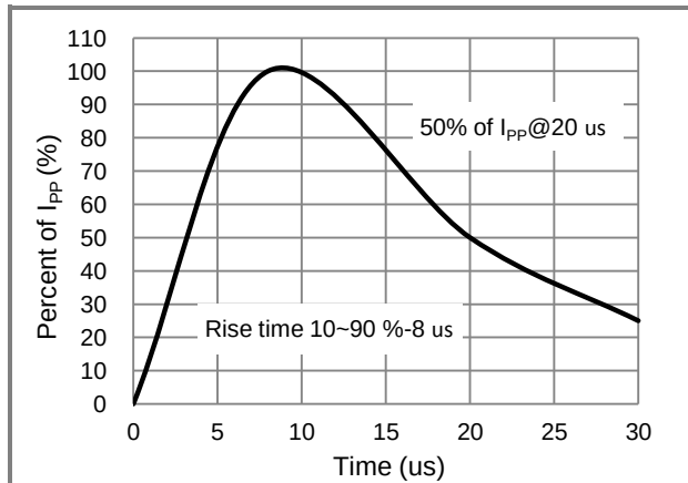
Fig.2 Pulse Waveform
