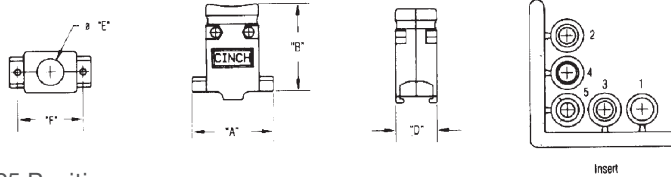
25 Position
