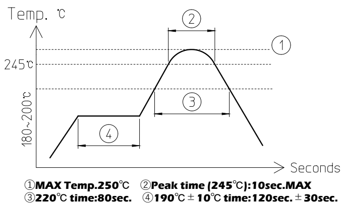
Fig 2. Reflow Profile
